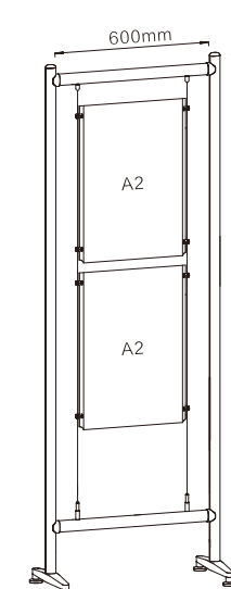
FS-01 (600X2000)A2 Order Number: 0468100721 Stand Size: 600X2000mm 2x A2 portrait poster holder 2x CF6-01 2x CF6-02 8x CVS-A or CVS-B 2x 2m 1.5mm cable
