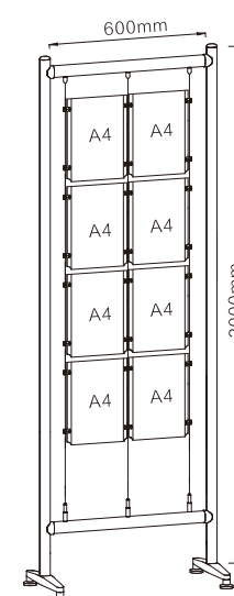
FS-01 (600X2000)A4 Order Number: 0468100121 Stand Size: 600X2000mm 8x A4 portrait poster holder 3x CF6-01 3x CF6-02 16x CVS-A or CVS-B 8x CVD 3x 2m 1.5mm cable
