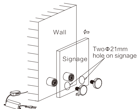
L-2525- 2 (2 sign standoffs +1 power)
