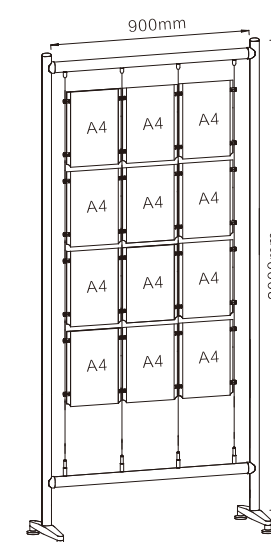
FS-01 (900X2000)A4 Order Number: 0468100221 Stand Size: 900X2000mm 12x A4 portrait poster holder 4x CF6-01 4x CF6-02 16x CVS-A or CVS-B 16x CVD 4x 2m 1.5mm cable
