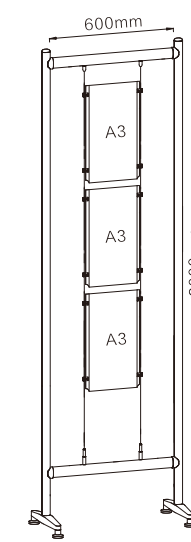
FS-01 (600X2000)A3 Order Number: 0468100421 Stand Size: 600X2000mm 3x A3 portrait poster holder 2x CF6-01 2x CF6-02 12x CVS-A or CVS-B 2x 2m 1.5mm cable
