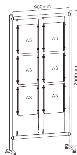
FS-01 (900X2000)A3 Order Number: 0468100521 Stand Size: 900X2000mm 6x A3 portrait poster holder 4x CF6-01 3x CF6-02 24x CVS-A or CVS-B 4x 2m 1.5mm cable
