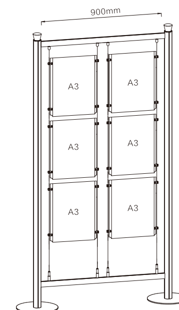
FS-02(900x2000)A3
