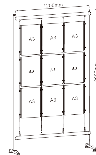
FS-01 (1200X2000)A3 Order Number: 0468100621 Stand Size: 1200X2000mm 9x A3 portrait poster holder 4x CF6-01 4x CF6-02 12x CVS-A or CVS-B 12x CVD 4x 2m 1.5mm cable
