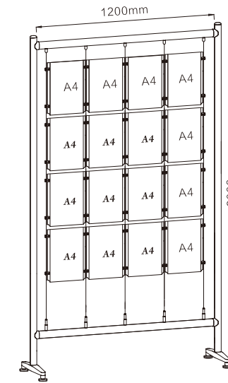
FS-01 (1200X2000)A4 Order Number: 0468100321 Stand Size: 1200X2000mm 16x A4 portrait poster holder 5x CF6-01 5x CF6-02 16x CVS-A or CVS-B 24x CVD 5x 2m 1.5mm cable
