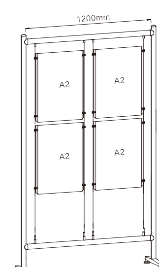
FS-01 (1200X2000)A2 Order Number: 0468100821 Stand Size: 1200X2000mm 4x A2 portrait poster holder 4x CF6-01 4x CF6-02 16x CVS-A or CVS-B 4x 2m 1.5mm cable
