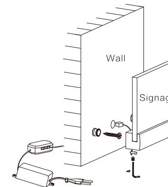
XC-80-1 ( 1 LED sign clamp + 1 power)
