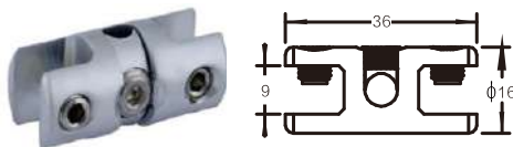
Double Clamp
